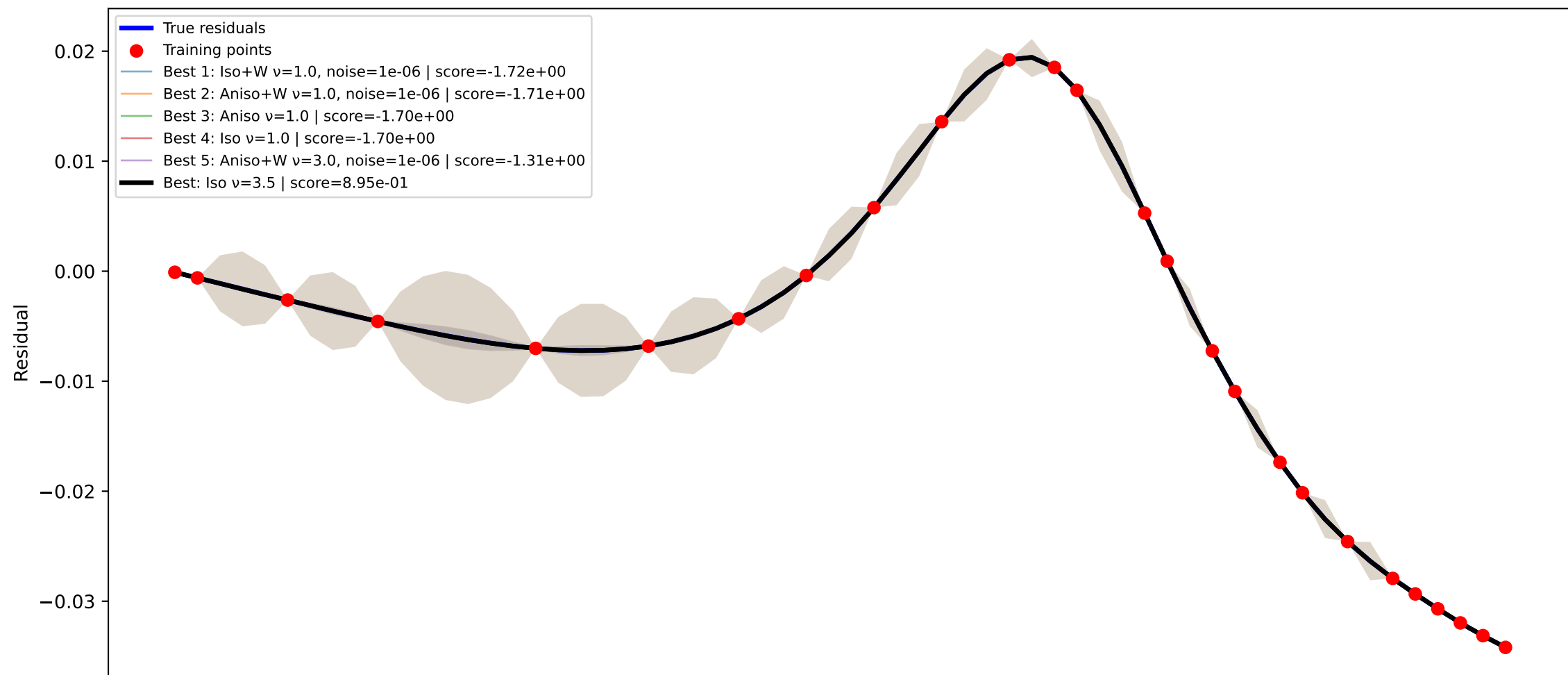
GPR kernel comparison node=3 RMSE=7.482e-06, train RMSE=1.047e-09
